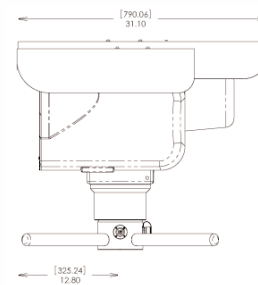
EOSS 825-S Side View
